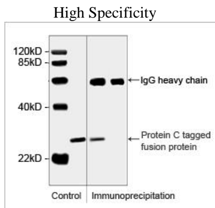
Fig 2. Western blot analysis of immunoprecipitates from Protein C tagged protein transfected CHO cell lysates. Protein C-tagged protein was immunoprecipitated with mouse anti-Protein C Tag mAb ( A01774 ).
