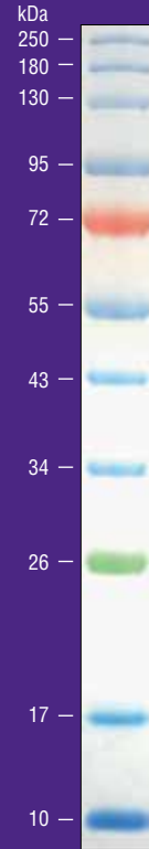
Color Prestained Protein Standard, Broad Range (10–250 kDa) 10–20% Tris-glycine SDS-PAGE Gel NEB #P7719
