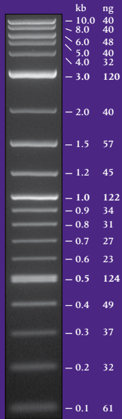
Quick-Load ® Purple 1 kb plus DNA Ladder (0.1 - 10.0 kb) - #N0550 1.0% TBE agarose gel. 1 µg/lane.
