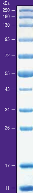
Blue Prestained Protein Standard, Broad Range (11–250 kDa) 10–20% Tris-glycine SDS-PAGE Gel NEB #P7718
